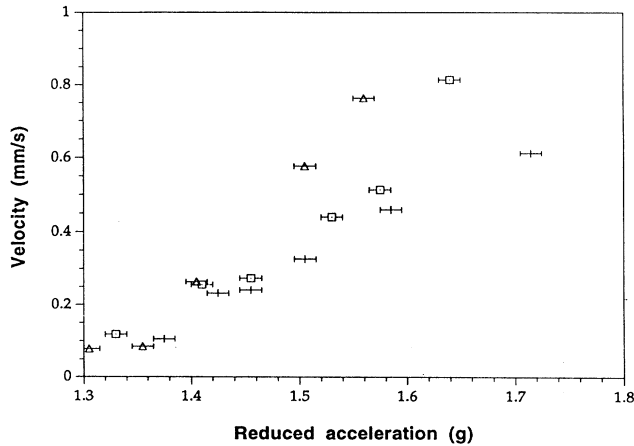
FIG. 10. Average rise velocity (from least-squares-fit line through the trajectories) against dimensionless acceleration. Crosses, squares, and triangles correspond to \Phi = 3, 7, and 12.5, respectively. An approximately linear rise in average velocity is observed for each case.
