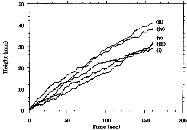
FIG. 5. Effect of initial intruder depth (measured to the top of the intruder) below the surface on the rise profile. (i) \Gamma=1.33\pm 0.01 , start depth=70 mm; (ii) \Gamma=1.28\pm 0.01 , start depth=60 mm; (iii) \Gamma=1.32\pm 0.01 , start depth=70 mm; (iv) \Gamma=1.37\pm 0.01 , start depth=60 mm; (v) \Gamma=1.35\pm 0.01 , start depth=75 mm. When the intruder reached 60 mm below the surface, the excitation was stopped, the surface was leveled, and the vibration then continued. In all cases the camera position was fixed, and filming took place when the intruder entered the field of view and the intruder height relative to the bottom of the field of view was plotted against time. One frame per cycle was taken.
