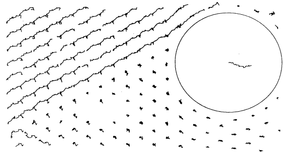
FIG. 16. Trajectory map showing the position of the background particles relative to the intruder disk. The intruder, with a size ratio, \Phi=7 , and its trajectory are also plotted. A reduced acceleration \Gamma=1.32 was used so that we are in the regime with intermittent rise characteristics. 32 frames were used to generate this plot, which captures a single slip plane-block motion event. Dots indicate the moving block of particles, which push the intruder upwards, and the particles on the left therefore fall away relative to the intruder. The figure has been rotated by 90^\circ so that the intruder moves from left to right across the page.
